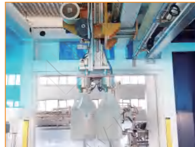
伺服式装箱机(气动抓手) Servo packing machine(Pneumatic gripper)
