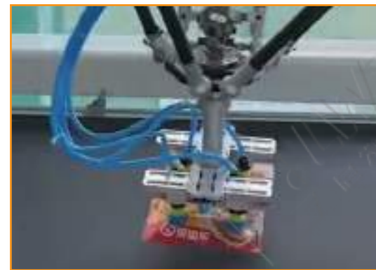
机器人装箱机 Robot packaging machine
